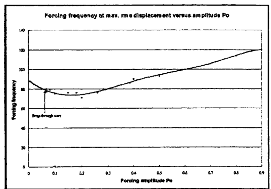
Fig. 11 Plot for \omega at max. q(rms) with p_o
