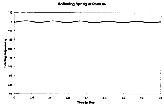
Fig. 12 Time history of softening spring behaviour
