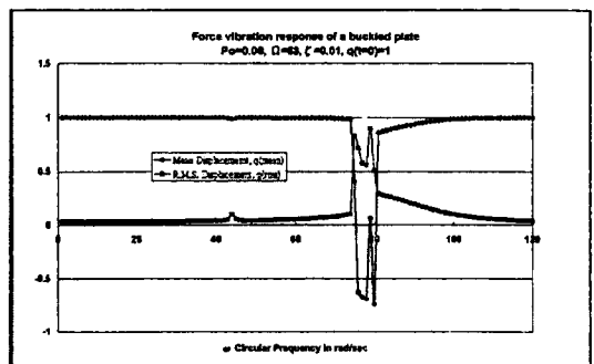
Fig. 5 Plot for chaotic behavior at 74 to 81 rad/s with p_0=0.08
