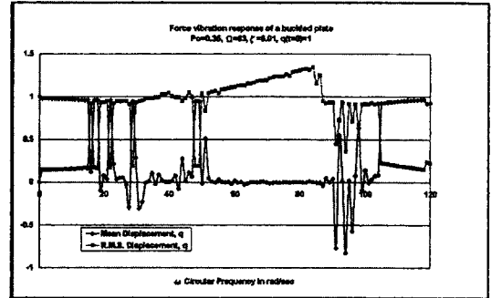
Fig. 7 Plot for chaotic behavior with p_o=0.35
