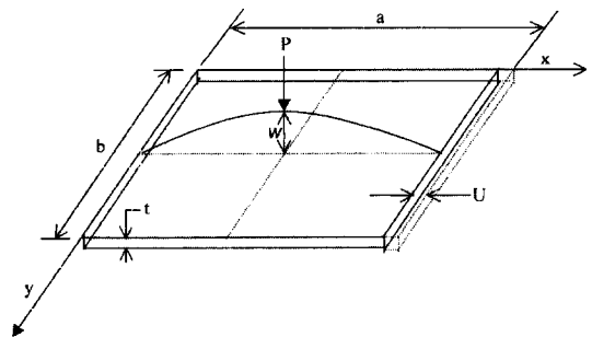
Fig. 1 Schematic diagram of a C-F-C-F plate model
