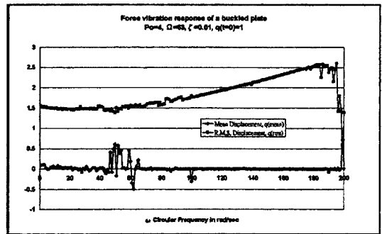
Fig. 9 Plot for hardening spring effect at p_o=4
