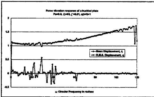
Fig. 8 Plot for hardening spring effect with p_o=0.9
