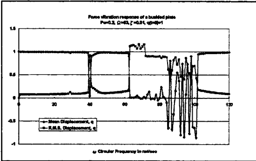
Fig. 6 Plot for chaotic behavior with p_o=0.2
